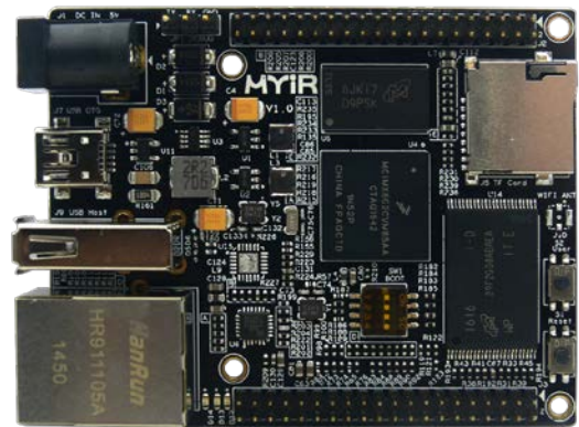
Figure 1-2 MYS-6ULX-IND
