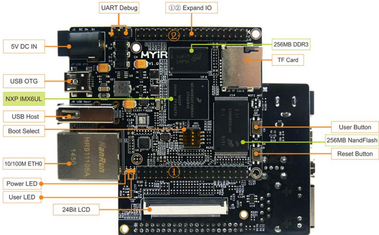
Figure 1-3 MYS-6ULX-IND
