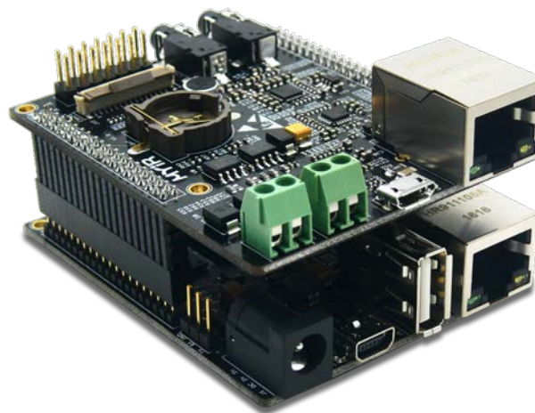
Figure 1-9 MYS-6ULX Connected with MYB-6ULX Base Board
